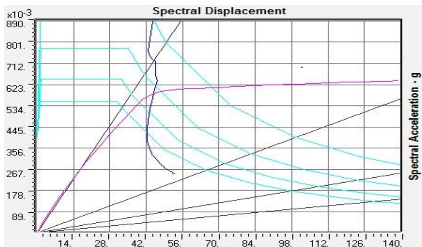
Figure 4. Showing capacity Spectrum
