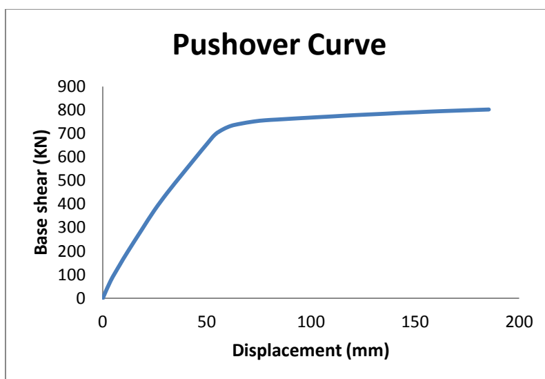
Fig 2. Showing Pushover curve of a building for four storey II zone
