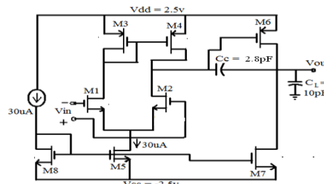
Fig. 3: Schematic of the error amplifier
