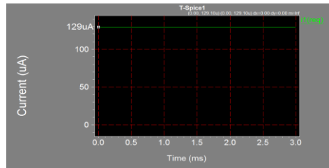
Fig. 7: quiescent current
