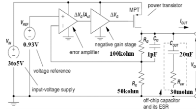
Fig. 5: complete design of power transistor(MPT) stage
