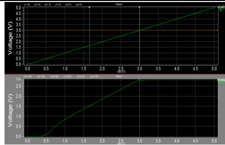
Fig. 6: drop out voltage
