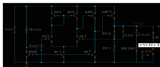
Fig 9: LDO with NMOS switch as load
