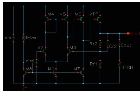
Fig. 2: Schematic of the proposed LDO regulator
