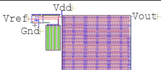
Fig. 14: proposed LDO full chip layout view
