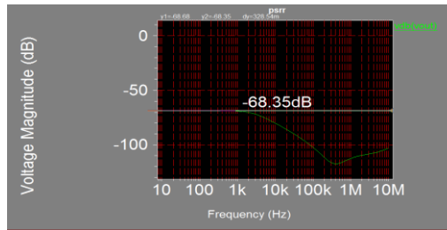
Fig.12: PSRR of proposed LDO
