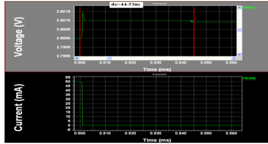
Fig.11: full load transient response
