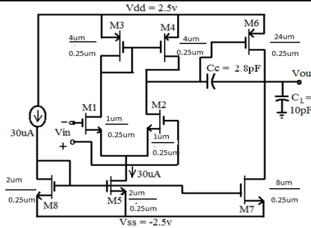
Fig. 4: design of two stage op amp
