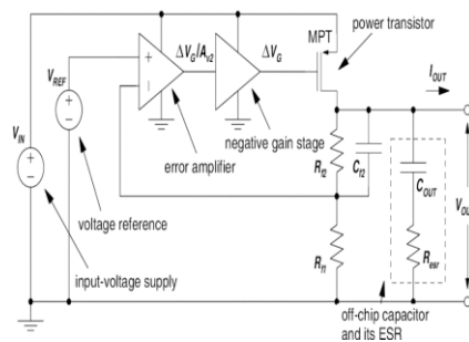
Fig. 1: circuit diagram of proposed LDO regulator
