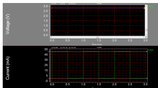
Fig. 10: load regulation
