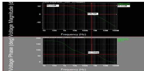
Fig. 13: gain and phase margin of the LDO
