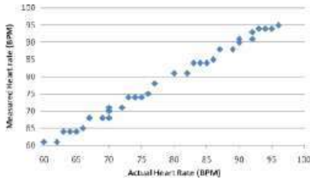
Fig. 10. The comparison of heart rate measurement.
