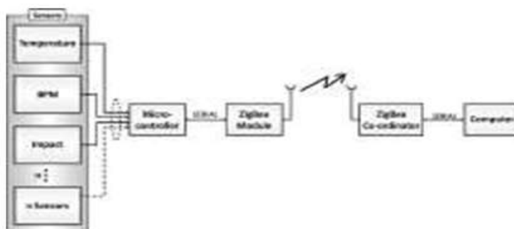
Fig. 1. Functional block diagram of system hardware.
