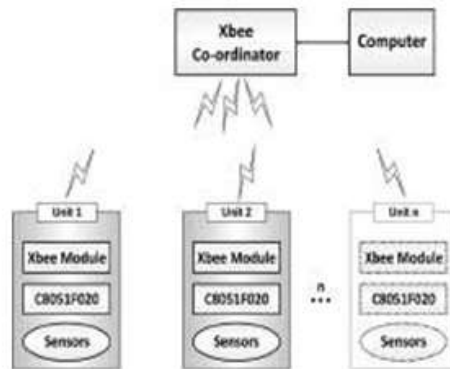
Fig. 14. System overview for wireless communication
