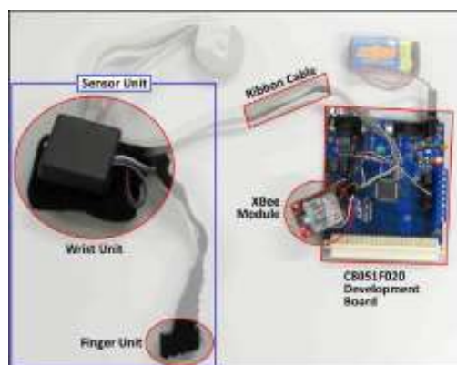
Fig. 19. Details of the prototype unit
