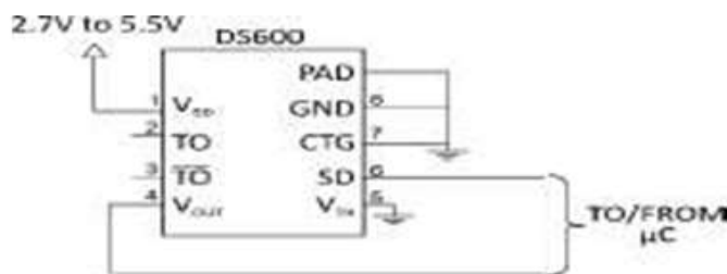
Fig. 2. Circuit application of DS600 temperature sensor.
