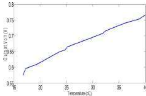
Fig. 3. Measured transfer characteristics of DS600.
