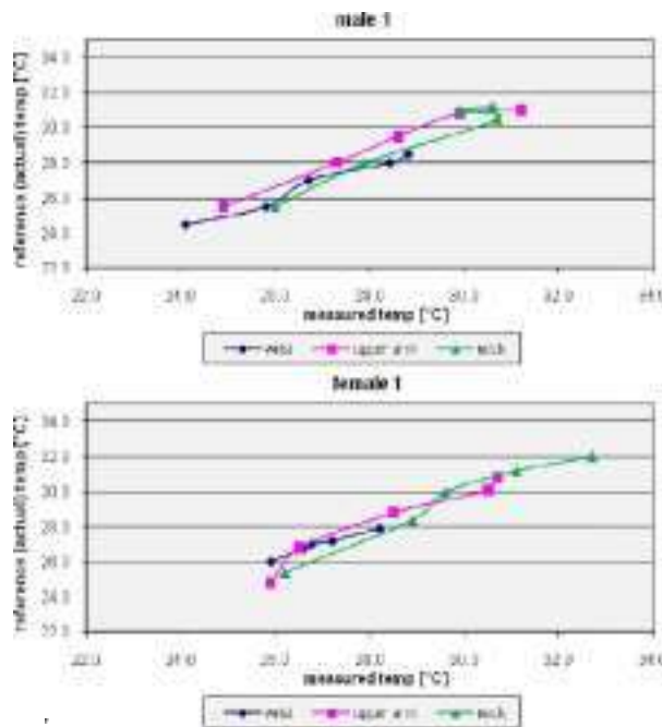
Fig. 4. The measured temperature of one male and one female.
