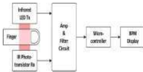
Fig. 6. Functional block diagram of the heart rate sensor [21].
