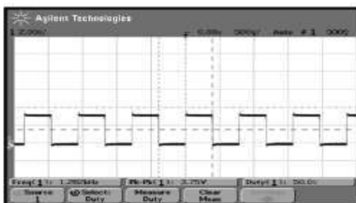
Fig. 11. Typical waveform of impact sensor in oscilloscope.
