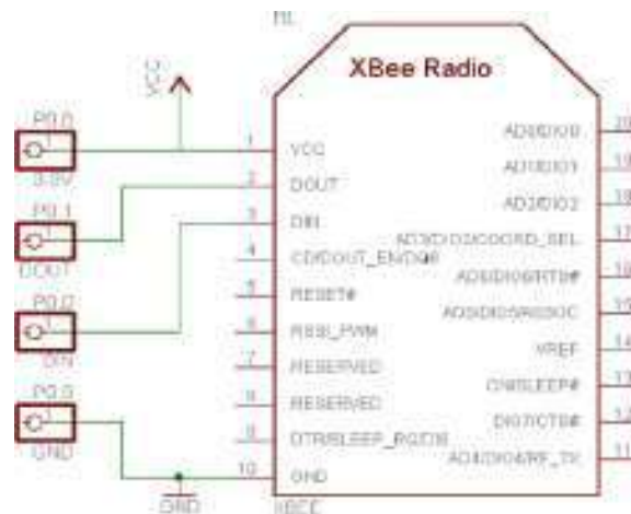
Fig. 15. Xbee module electrical connection with microcontroller.
