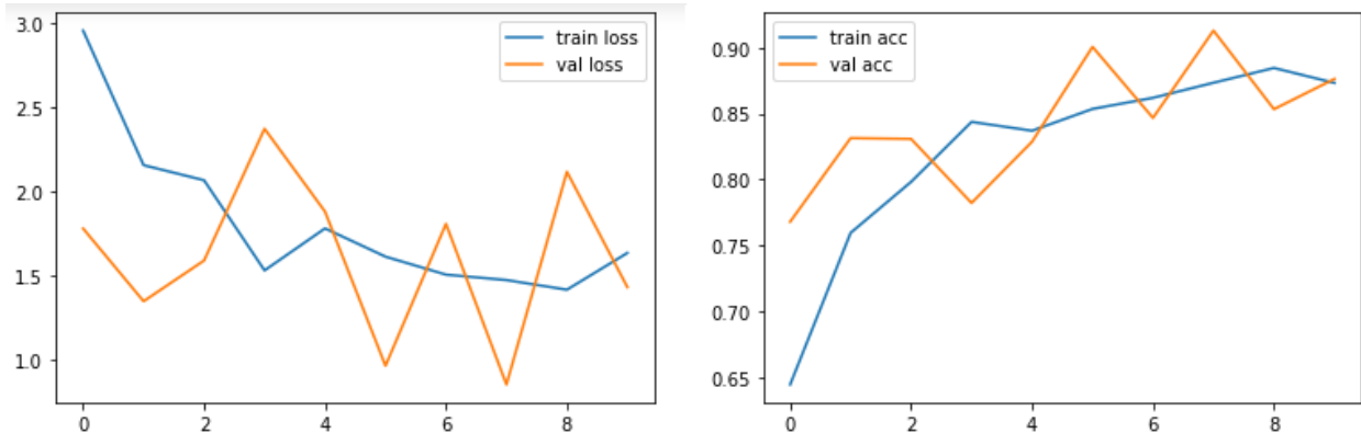
Fig.4: Accuracy Graph
