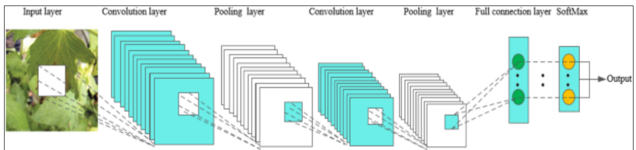
Fig.2: Convolutional Neural Network
