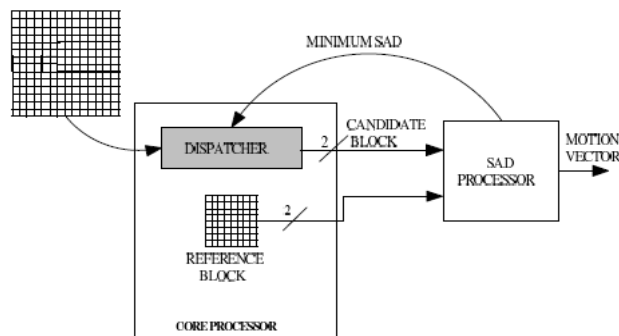
Figure 8 Core Processor Communication with SAD
