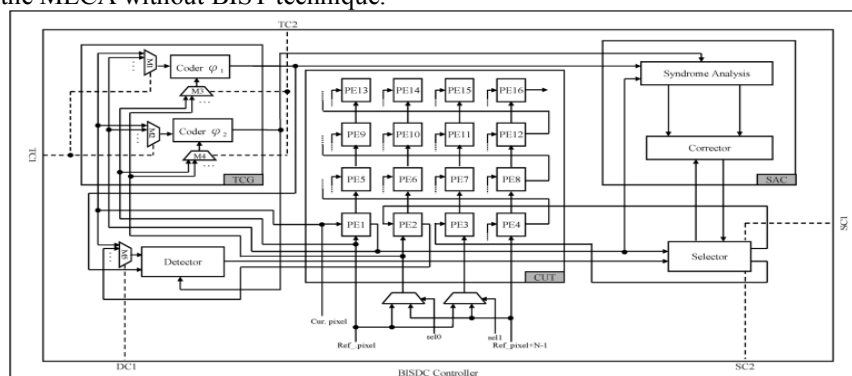
Fig1: Block Diagram of Proposed MECA BISDC.
