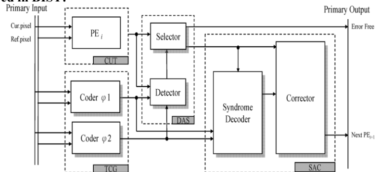
Fig 1 Example of the self-detection/correction operations
