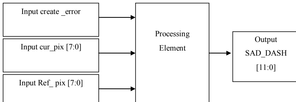
Fig 3 Processing Element Module Schematic Diagram
