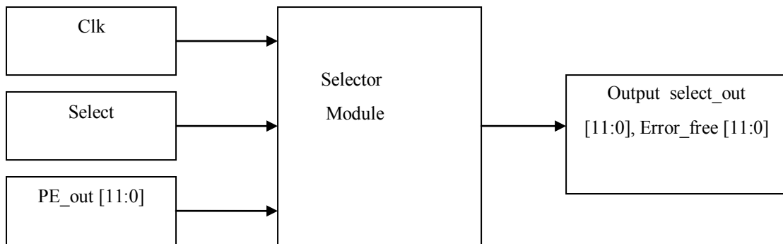
Fig 5 Selector Module Schematic diagram
