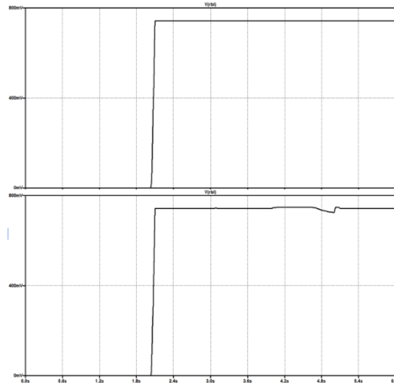
Fig. 9. 20T TICE's RBL value without any error and with a 1-0 bit error while reading a stored value of 1
