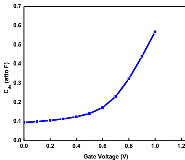
Figure 8 Drain-to-source ( C_{ds} ) capacitance at 4 nm dielectric thickness
