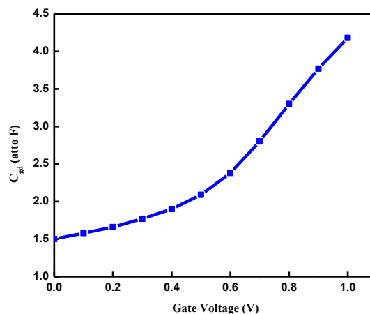
Figure 6 Gate-to-drain ( C_{\text{gd}} ) capacitance at 4 nm dielectric thickness
