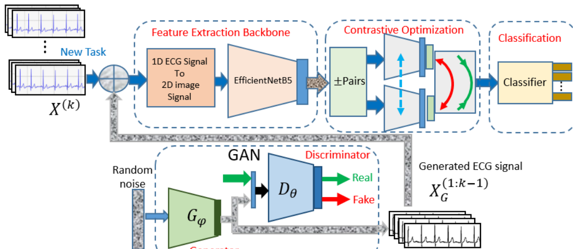
Figure1. Contrastive learning and GAN based hybrid model.
