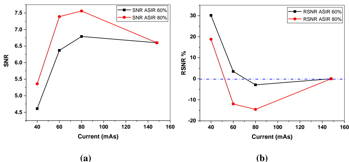
Fig 5: variation of (a) SNR and (b) percentage reduction of SNR associated with different reduced currents.
