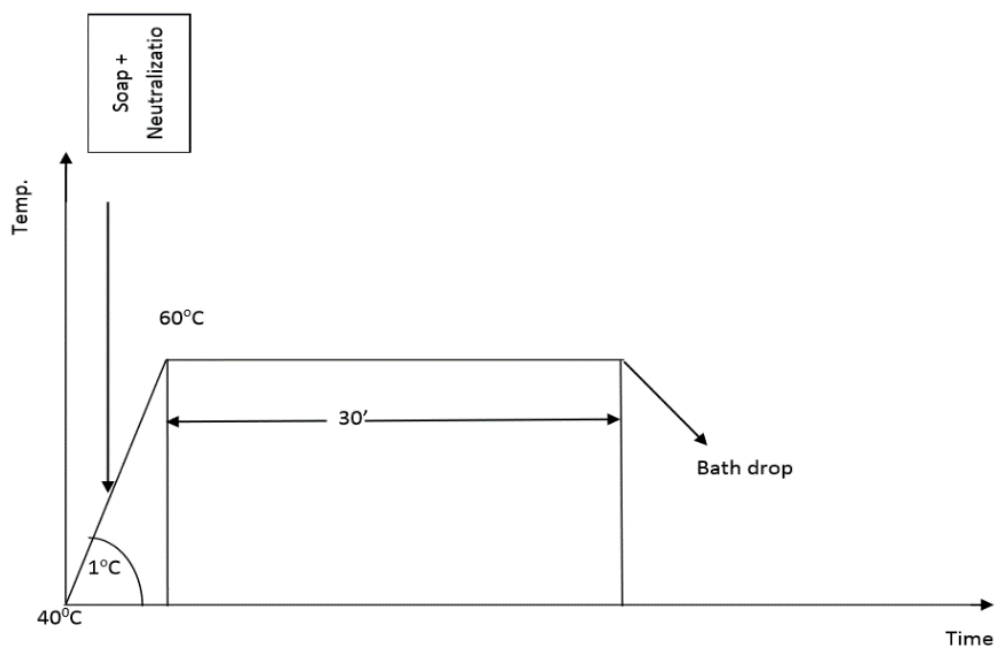
Curve 1.3 Hot wash & soaping
