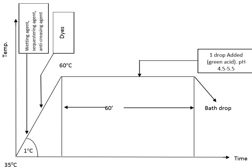
Curve 1.2: Dyeing process curve
