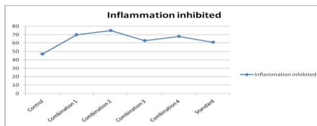
Graph 1: The graph shows the percent inflammation inhibited by the various combinations.
