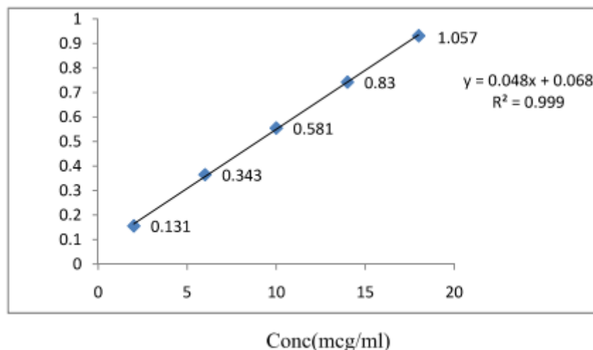
Figure 2: Calibration Curve of Lamivudine
