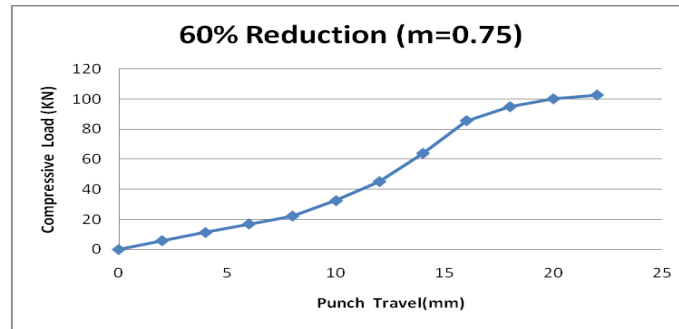
Fig 3.4 Compressive Load vs Punch Travel graph for 60% reduction(m=0.75)
