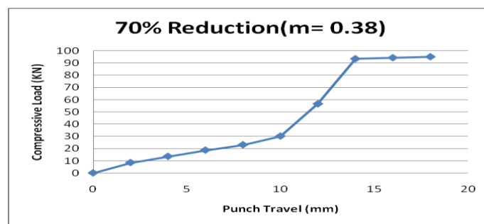
Fig 3.2. Compressive Load vs Punch Travel graph for 70% reduction(m=0.38)
