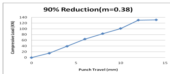
Fig 3.3. Compressive Load vs Punch Travel graph for 90% reduction(m=0.38)
