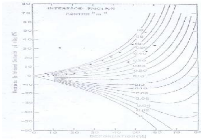
Fig 2.4. theoretical calibration curve for standard ring 6:3:2 [21]
