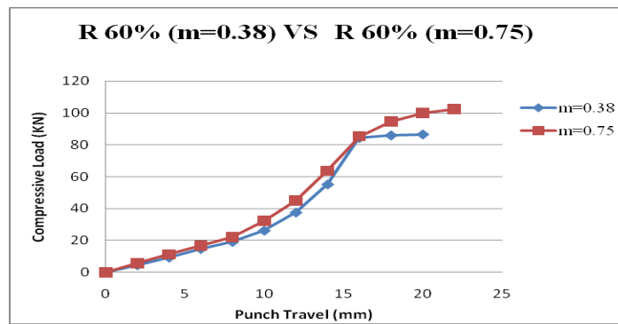
Fig 3.5 Comparison of R 60% (m=0.38) with R 60% (m=0.75)
