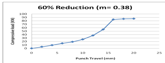
Fig 3.1. Compressive Load vs Punch Travel graph for 60% reduction (m=0.38)
