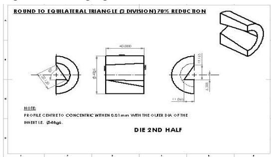
Fig 2.6. Converging die with 70% reduction
