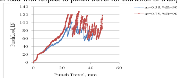
Fig. 4.3 variation of punch load with respect to punch travel for extrusion of Triangular section (90% reduction)
