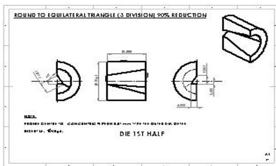
Fig 2.7. Converging die with 90% reduction
