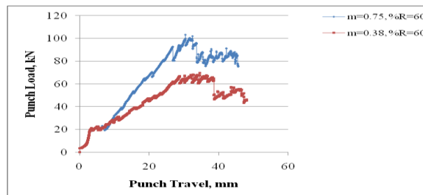
Fig.4.1 variation of punch load with respect to punch travel for extrusion of triangular section (60% reduction)
