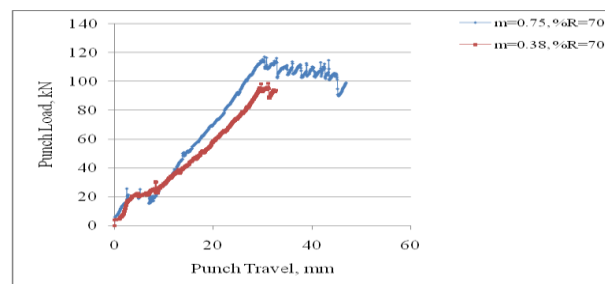
Fig. 4.2 variation of punch load with respect to punch travel for extrusion of triangular section(70% reduction)
