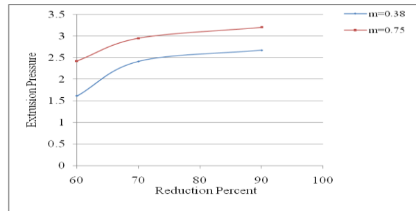
Fig. 4.4 comparison of wet and dry extrusion pressure for extrusion of triangular sections. It is indicated that the extrusion pressure increases with increase in reduction and friction factor. It is observed that the extrusion pressure is higher for dry friction.
