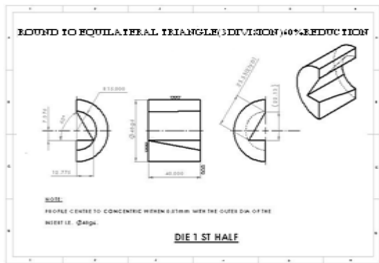
Fig 2.5. Converging die with 60% reduction
