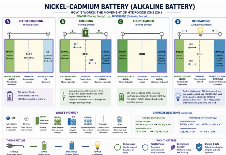
Figure 11: There are four possible stages of operation shown graphically for the Ni-Cd battery (AI generated)
