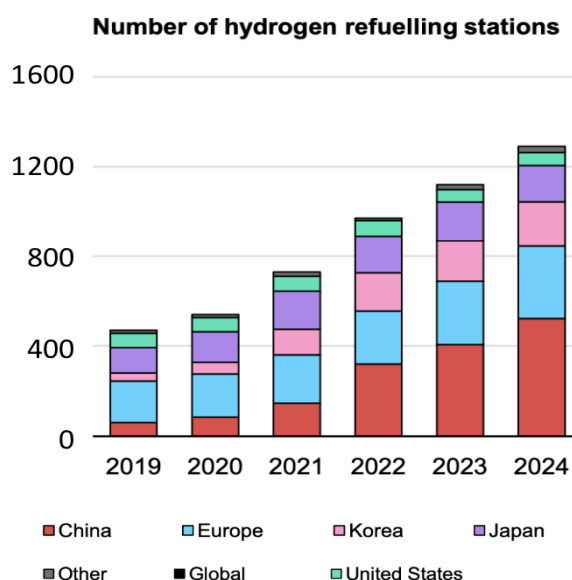
Fig-2: Hydrogen refuelling stations in different regions of the world
