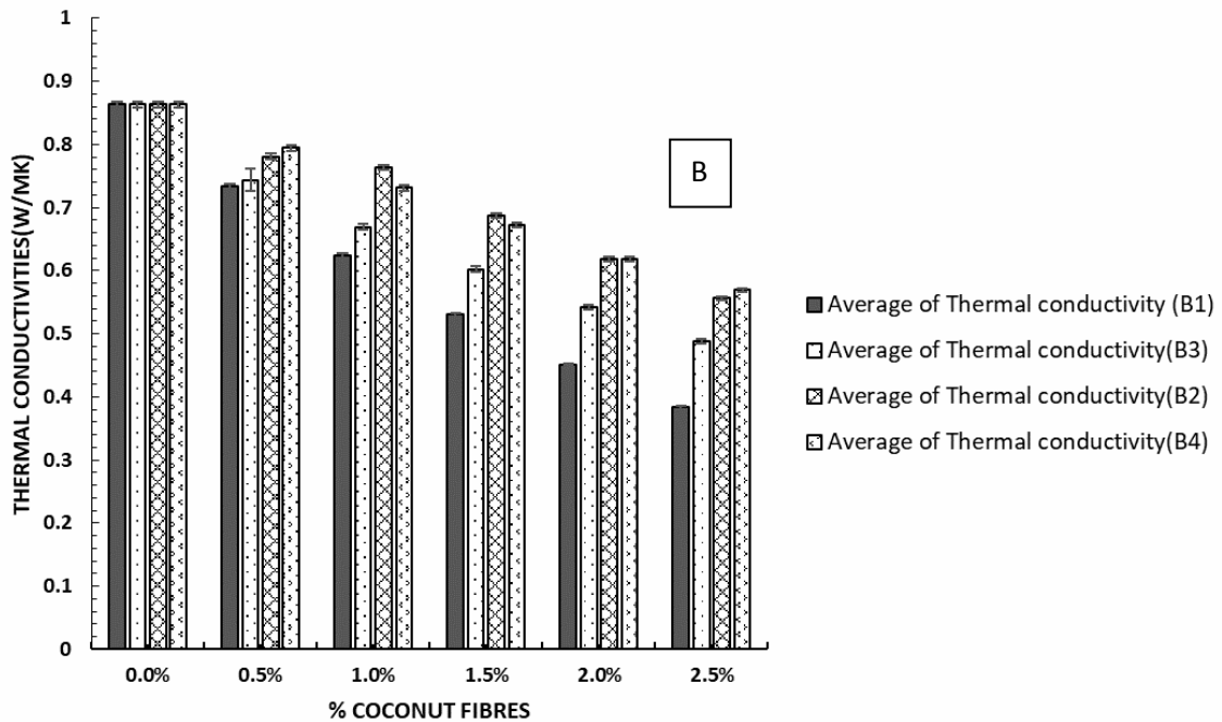
Figure 13: Thermal conductivity of bricks as function of (A) spikelet fibres (%) and (B) coconut fibres (%)
