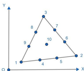
Figure 2.1: Triangular domain subdivided into one cubic element
