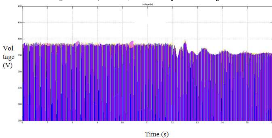
Fig 10. Voltage of μG for WT, MT and Battery with load change
