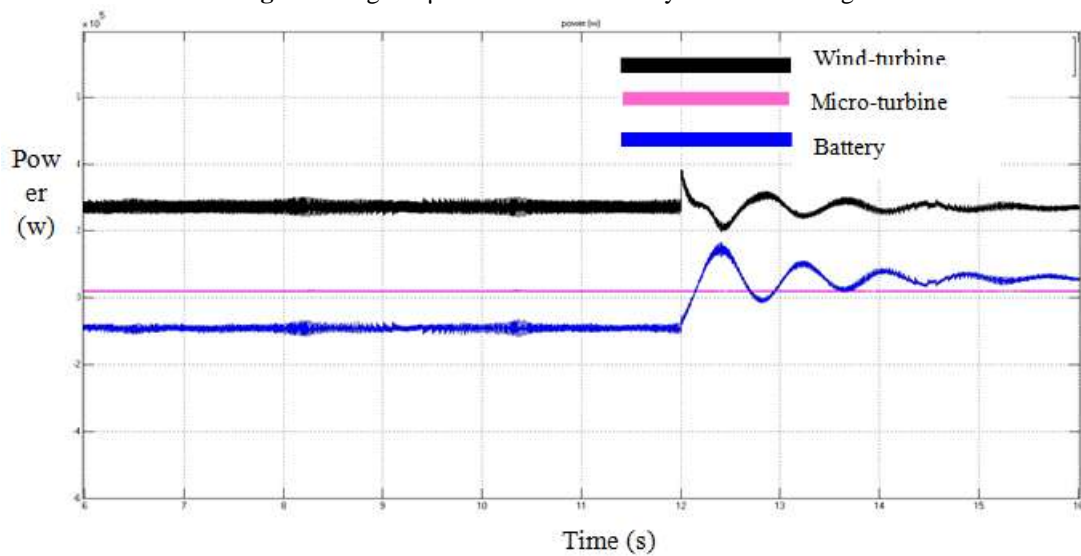
Fig 9. Power of μG for WT, MT and Battery with load change
