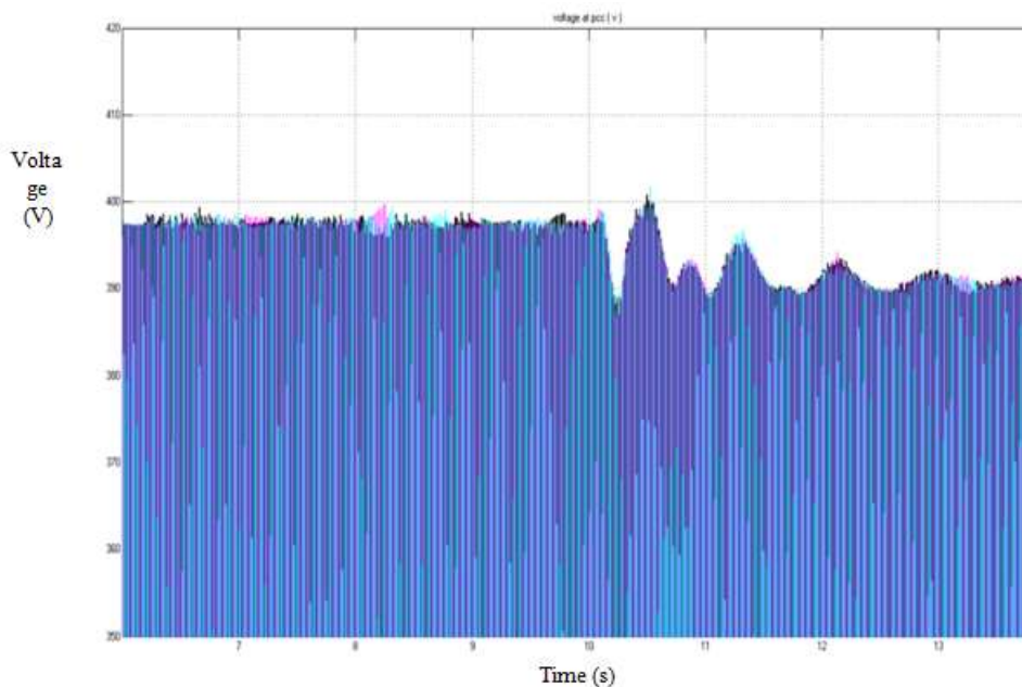
Fig 4. Voltage of \mu G for WT and Battery with wind speed change
