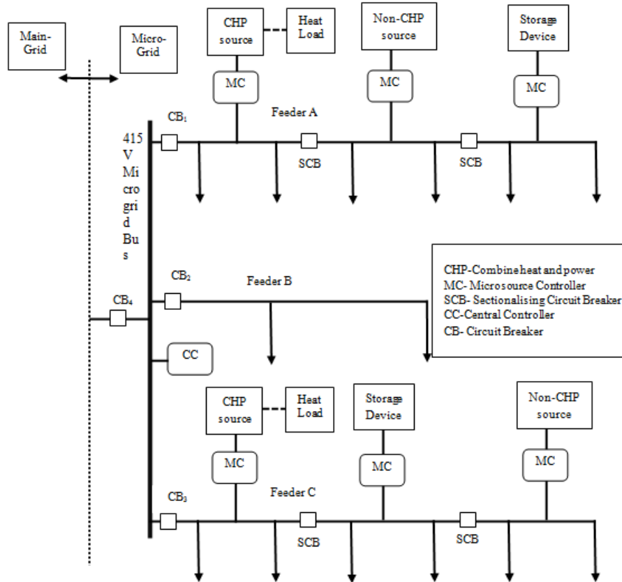
Fig 1. Typical Configuration of a \mu G [1].
