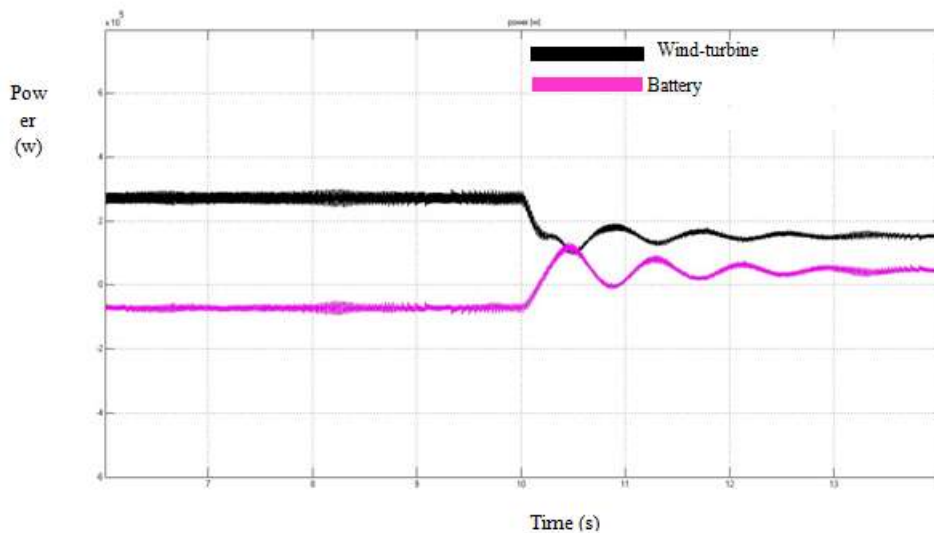
Fig 3. Power of \mu G for WT and Battery with wind speed change.
