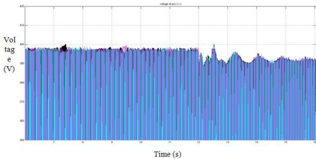
Fig 8. Voltage of μG for WT and Battery with load change
