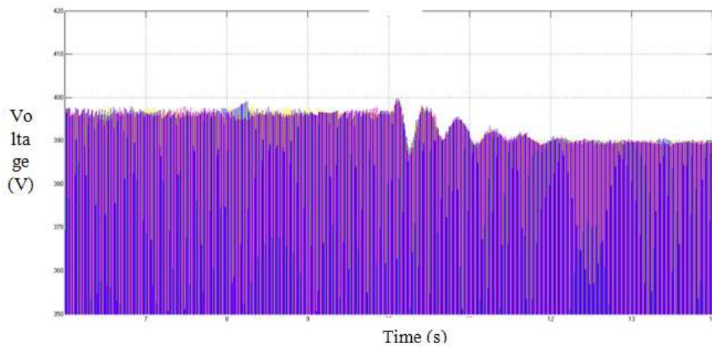
Fig 6. Voltage of \mu G for WT, MT and Battery with wind speed change
