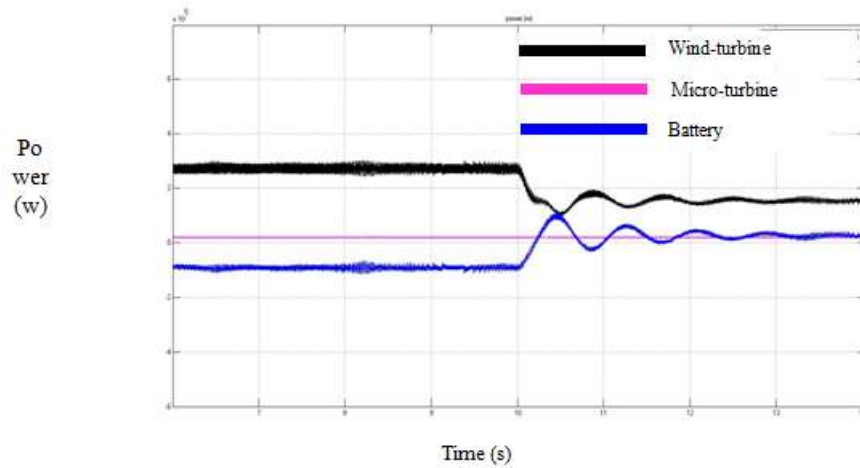
Fig 5. Power of \mu G for WT, MT and Battery with wind speed change.
