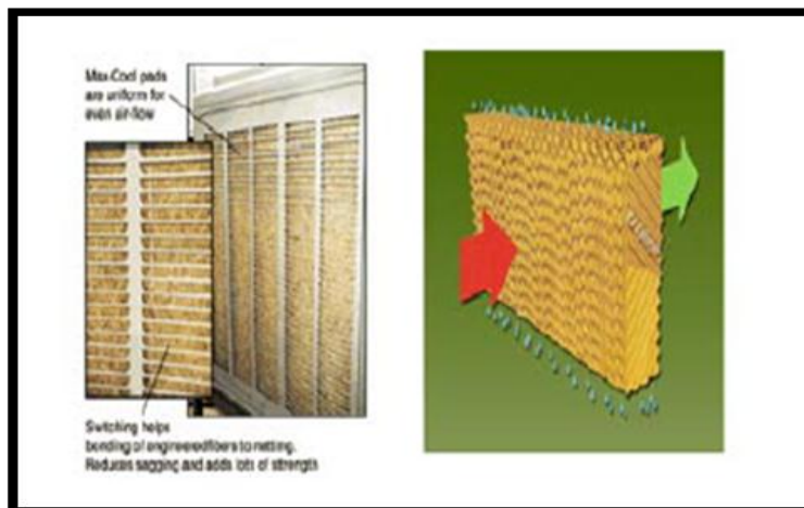
Fig. 2 Cooling Pad
