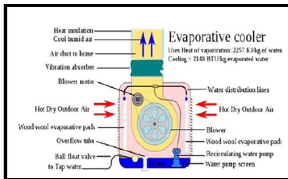
Fig. 1 Working Principle
