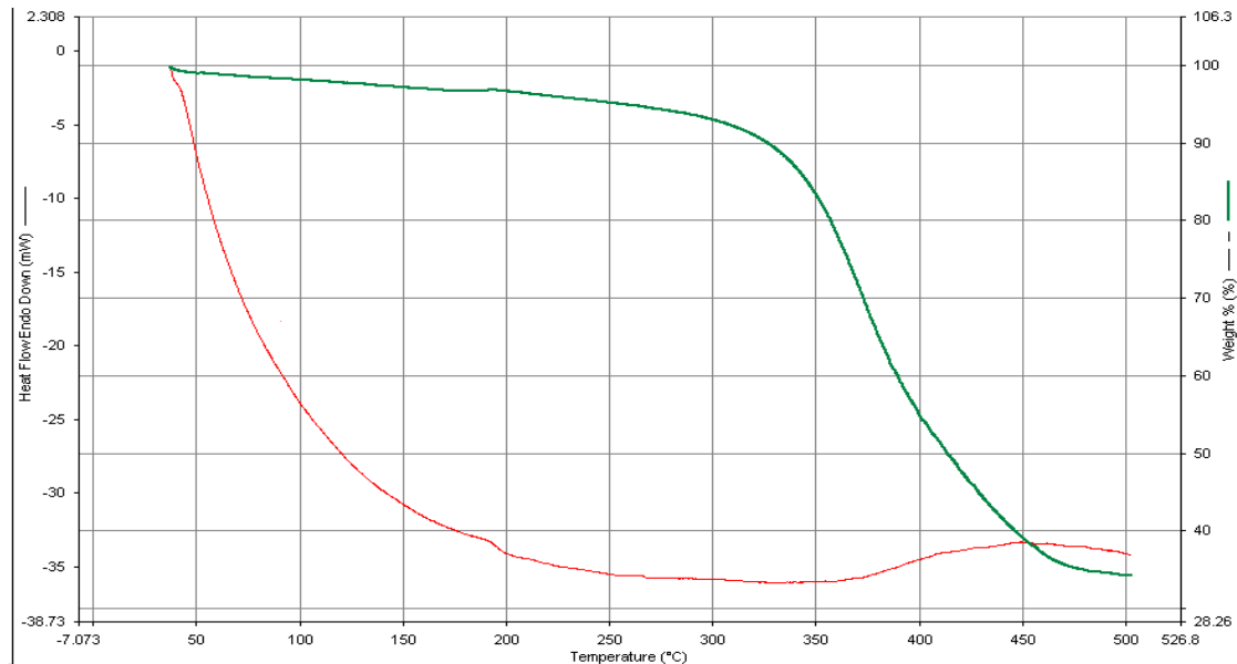
Figure 2: TGA and DSC analysis of 40% fly ash epoxy composite
