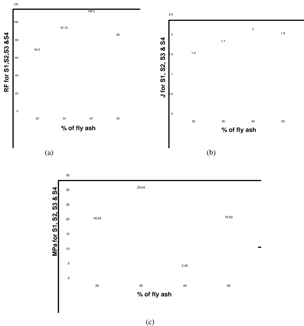
Figure 1: Variation of a) hardness b) toughness and c) tensile strength with percentage of fly ash in fly ash-epoxy resin composite
