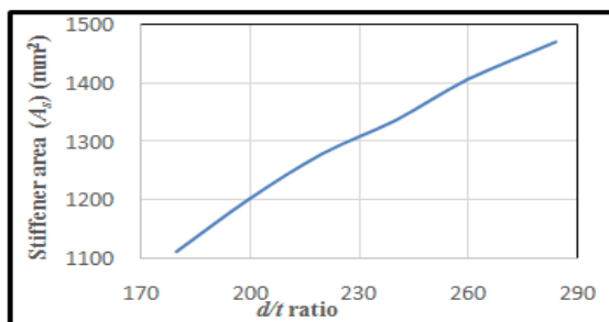
Figure 5: The relationship between web depth-to-thickness ratio and the vertical stiffener cross-section area
