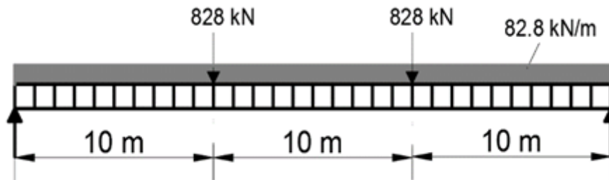
Figure 1: Plate girder loading
