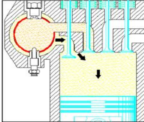
Figure: Release of pure air into cylinder
