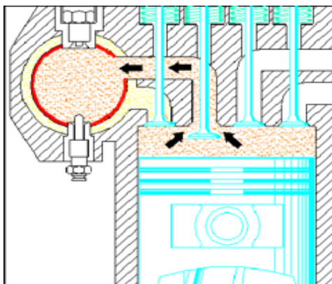
Figure: Recompression of the pure air in chamber
