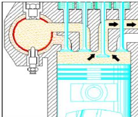
Figure: Exhaust of combustion gases
