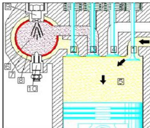
Fig: Intake of pure air in cylinder
