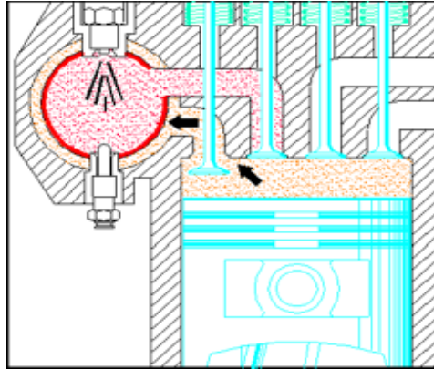
Figure: Compression of pure air in heating chamber
