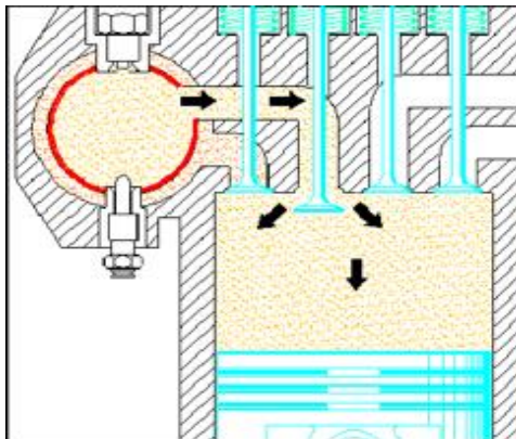
Figure: Release of combustion gases in the cylinder
