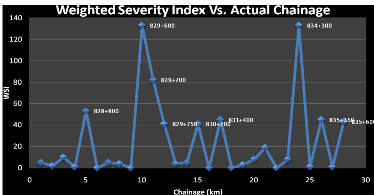
Graph 4 : Above graph shows the variation of WSI along the study area. WSI exceeding 40 is considered as very high and those chainages are written at respective points in above graph. (eg. 828+800 means 828.800km actual chainage).
