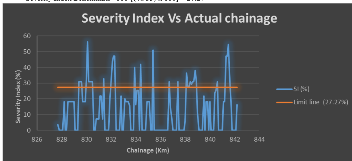
Graph 1 : Above graph shows the relationship of Severity index and actual chainage. The blue line indicates severity index and the orange line indicates the limit for severity index. Severity index more than 27.27 is considered as very high.
