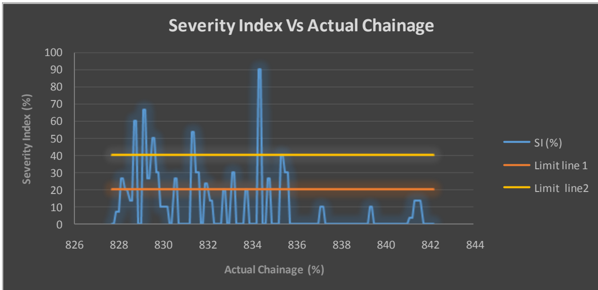
Graph 2 : Above graph shows the relationship between severity index and actual chainage. Blue line indicates the severity index. Orange and yellow lines are the limit lines. Severity index between the two limit lines is high and that beyond 40 is very high.
