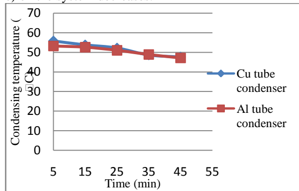
Fig.3: Variation in air outlet temperature of condensers Fig.4: Variation in condensers condensing temperature Figure 4 shows the variation in condensing temperature. Condensing outlet temperature is depends on temperature of compressor and it's given at the end of the condenser circuit. When the heat is transferred from refrigerant to air the vapour refrigerant gets condensed upto saturation temperature which is relevant to the compressor pressure and also degree of sub-cooled below the saturation temperature to get more refrigerating effect to improve efficiency. It is observed that the condensing outlet temperature of condenser is same for Cu as well as Al. It means the heat rejection capacity of both the condenser is same.
