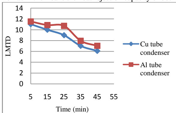
Fig.5: Variation in LMTD of condensers
