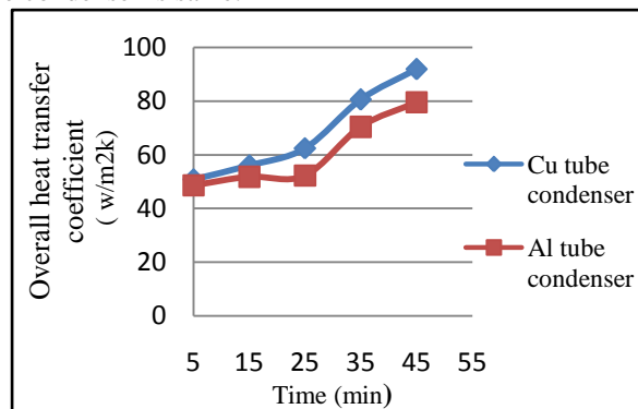
Fig.6: Variation in overall heat transfer coefficient of Condensers
