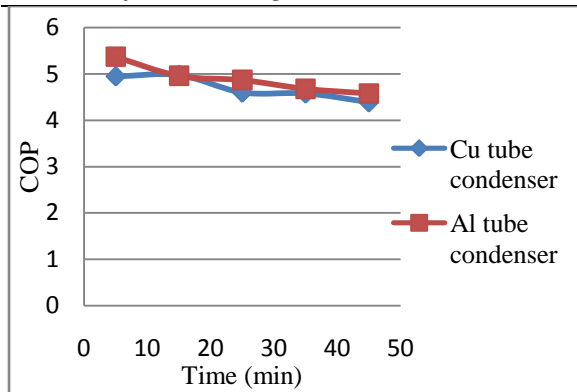
Fig 7: Variation in COP of condensers
