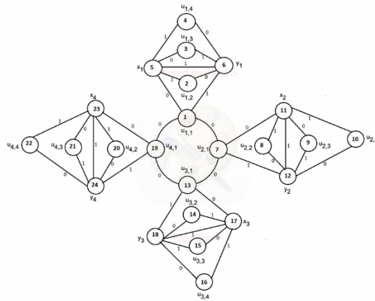
Figure 6. C(4, (+\Gamma(Z_9)))
