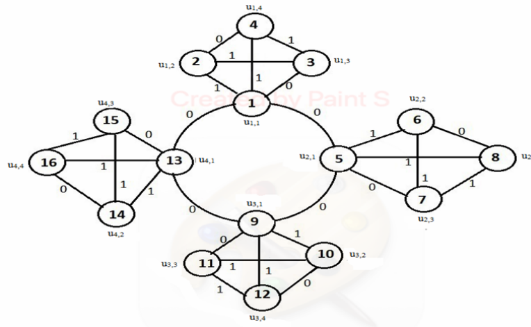
Figure 4. C (4,Γ 0)
