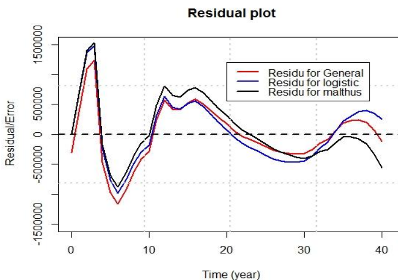
Figure 2: The plot for residuals of the models
