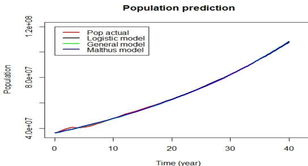
Figure 1: Time versus the predicted population
