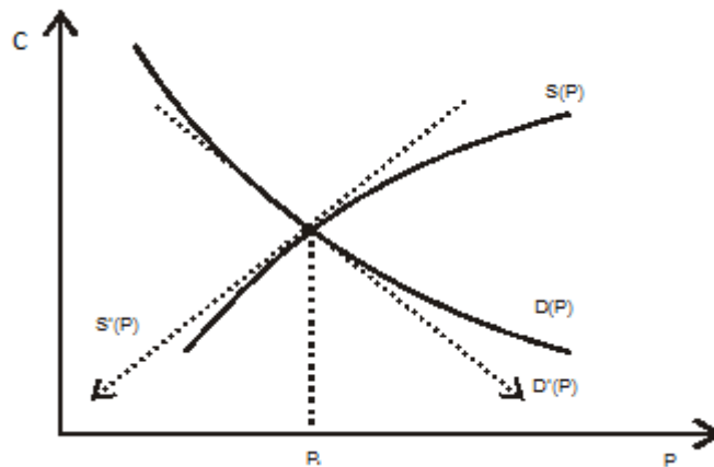
Fig 6 : Unique equilibrium value of P .
