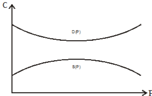
Fig 4 : Demand exceeds supply for every price.
