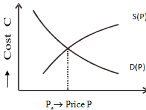
Fig 1 : The usual plot of demand D(P) and supply S(P) giving the equilibrium price P , where they meet.
