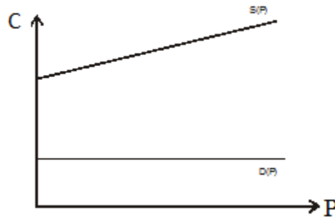
Fig 2 : Supply and demand curve where the equilibrium value is zero.
