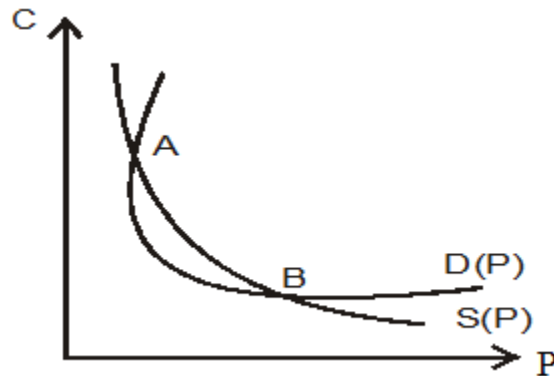
Fig 5 : The aggregate supply S(P) is decreasing and there are two equilibrium values of P .
