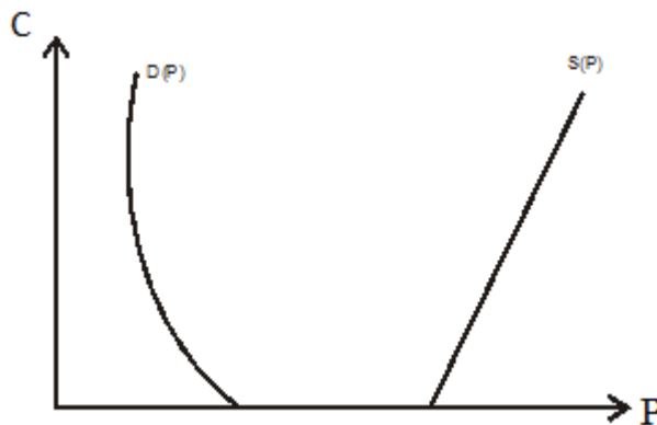
Fig 3: Supply and demand must both be zero for equilibrium here.
