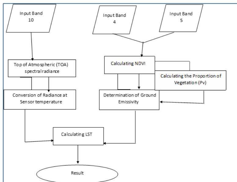
Figure 3. Algorithm for SUHI Evaluation And Assessment Source: Avdan & Jovanovska (2016)
