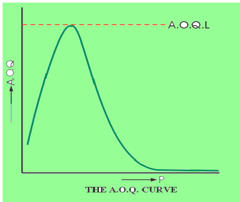
Figure 4: A.O.Q. Curve
