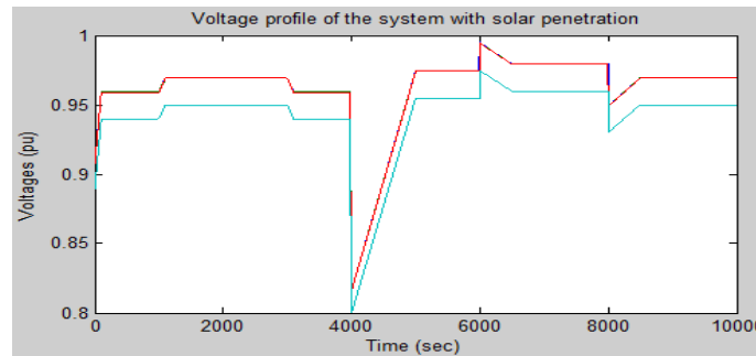
Fig.7: Voltage profile of the system with solar penetration.
