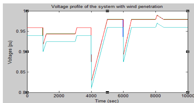
Fig.6: Voltage profile of the system with wind penetration.
