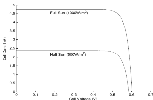
Fig.4. I-V plot of ideal PV cell under two different levels of irradiance (25°C).
