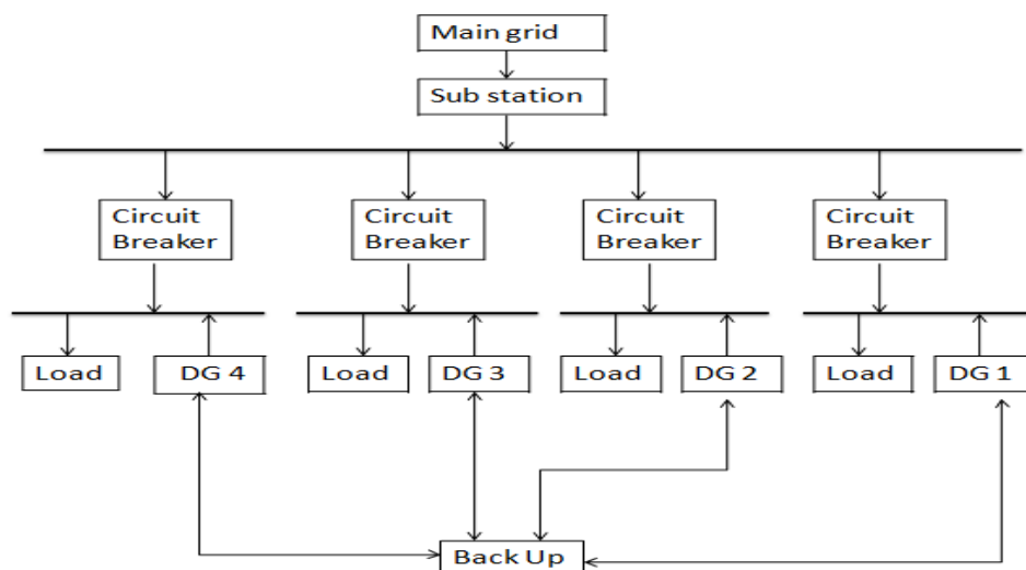
Fig. 5: A Modified Benchmark Micro grid test system.
