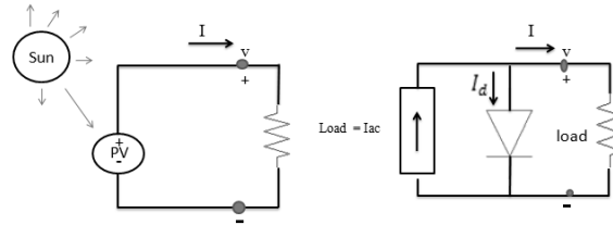
Fig.3 (a): PV cell with a load and its simple equivalent circuit.
