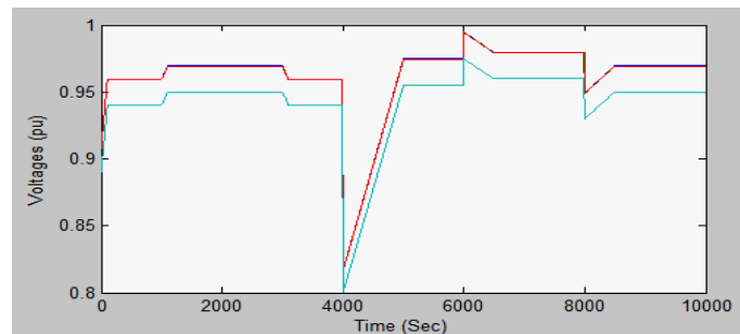
Fig.8: Voltage profile of the system with both solar & wind penetration.
