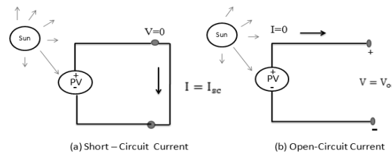
Fig.3 (b): Diagrams showing a short-circuit and an open-circuit condition
