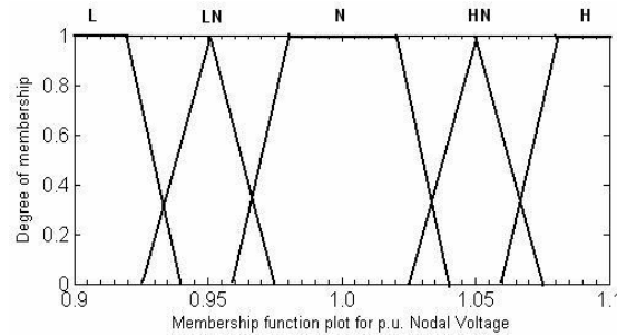
Figure-2. Membership function plot for p.u. nodal voltage.
