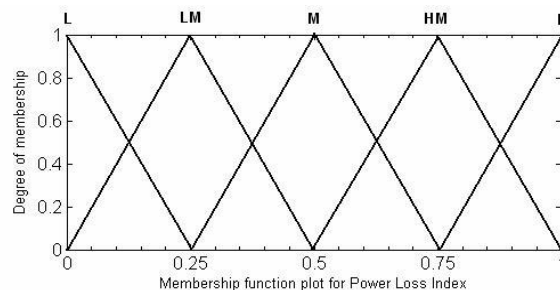
Figure-1. Membership function plot for P.L.I.
