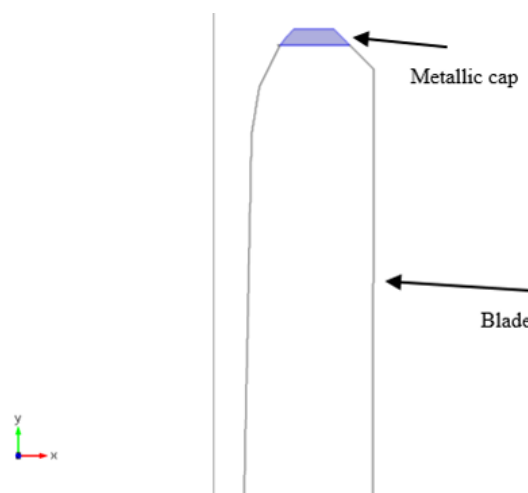
Fig. 5 Metallic Cap Method [37]
