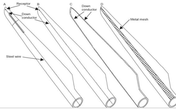
Fig. 8 Lightning protection methods on the blade. (A and B, Receptor Method), (C, Metallic Conductor on the Blade Edges), (D, Metallic Mesh). IEC 61400-24
