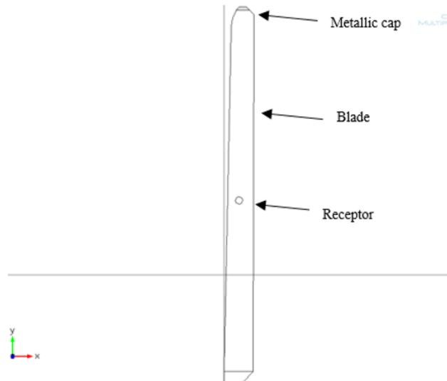
Fig. 6 Enhanced Method [39]
