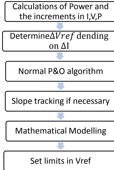
Fig. 2. Flow charts for the slope tracking P&O algorithms
