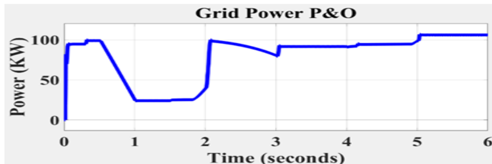
(a) Normal P&O
