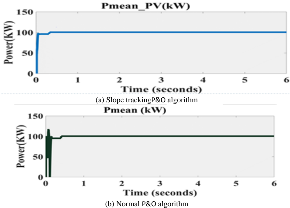
Fig. 4. Output power from solar PV power system at STC
