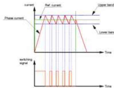
Figure 14. Hysteresis controller
