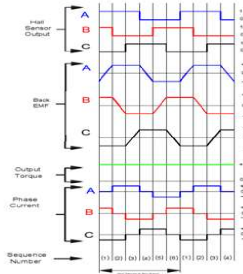
Figure 3. Wave forms of Hall sensors, BEMF, torque and phase currents
