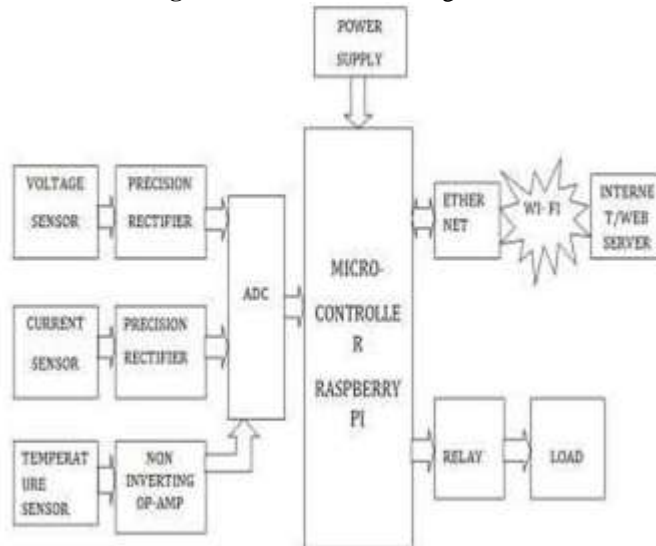
Figure 1: Server Block Diagram
