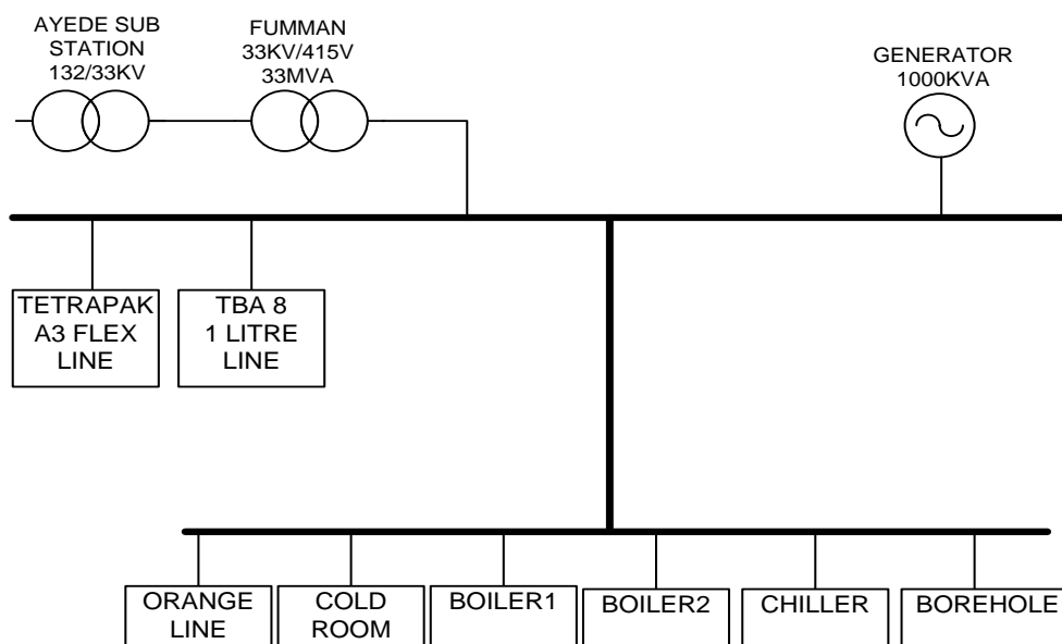
Figure 4: The FUMMAN Agricultural Products Industries PLC Layout
