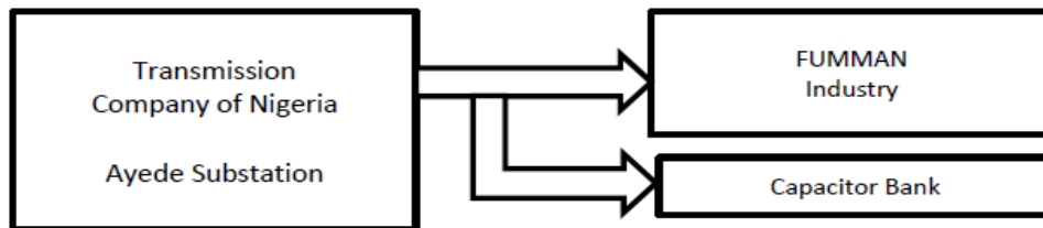
Figure 1: The methodology
