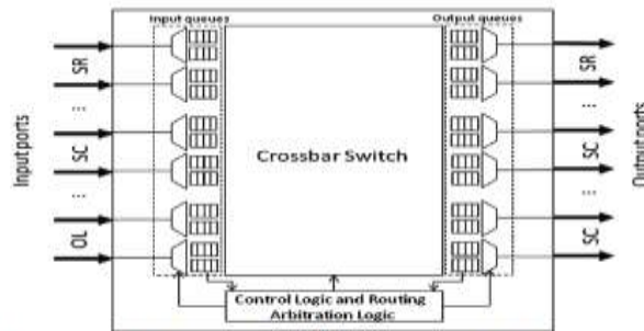
Figure 2. NoC router scheme including input and output registers, crossbar switch and routing and arbitration logic.
