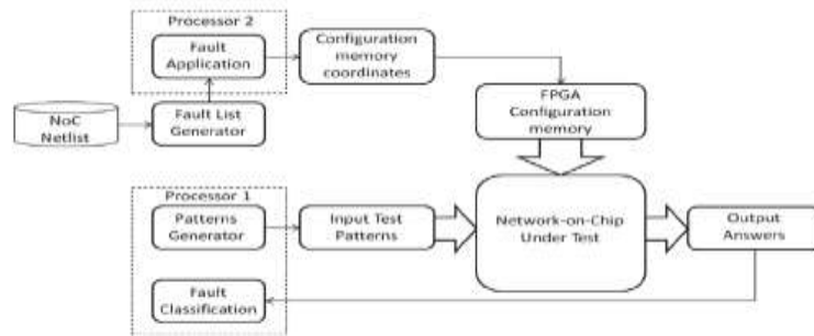
Figure 3. The fault injection execution flow of the proposed method.
