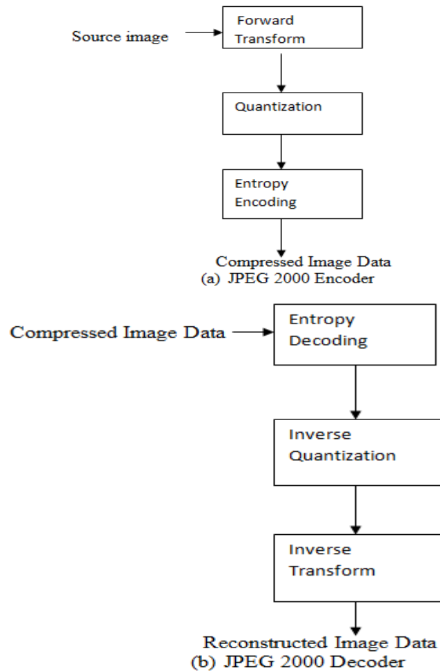
Figure 2. General block diagram of JPEG 2000
