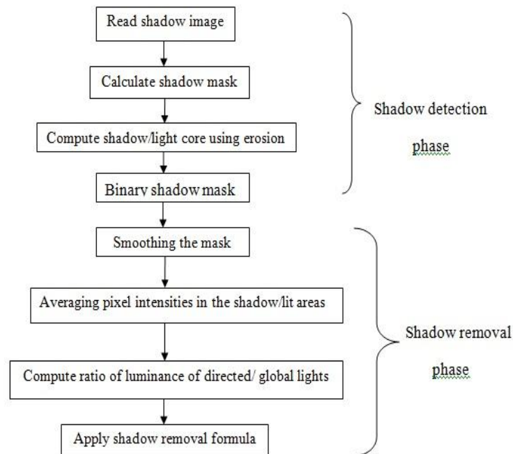
Fig 2. Block diagram of proposed approach.
