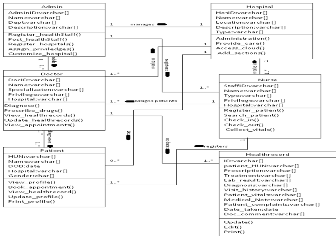
Figure 3.2: Class Diagram of the proposed system
