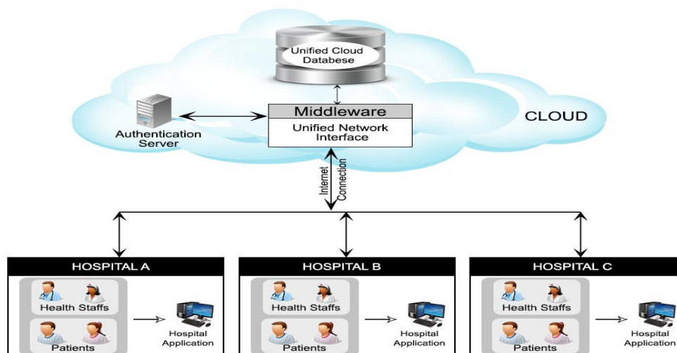
Figure 3: The Architecture of the PC-CBEHR System
