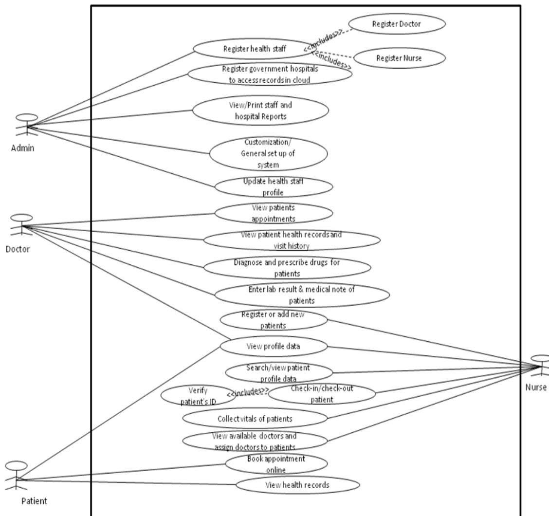
Figure 1: The Use Case Diagram of the System
