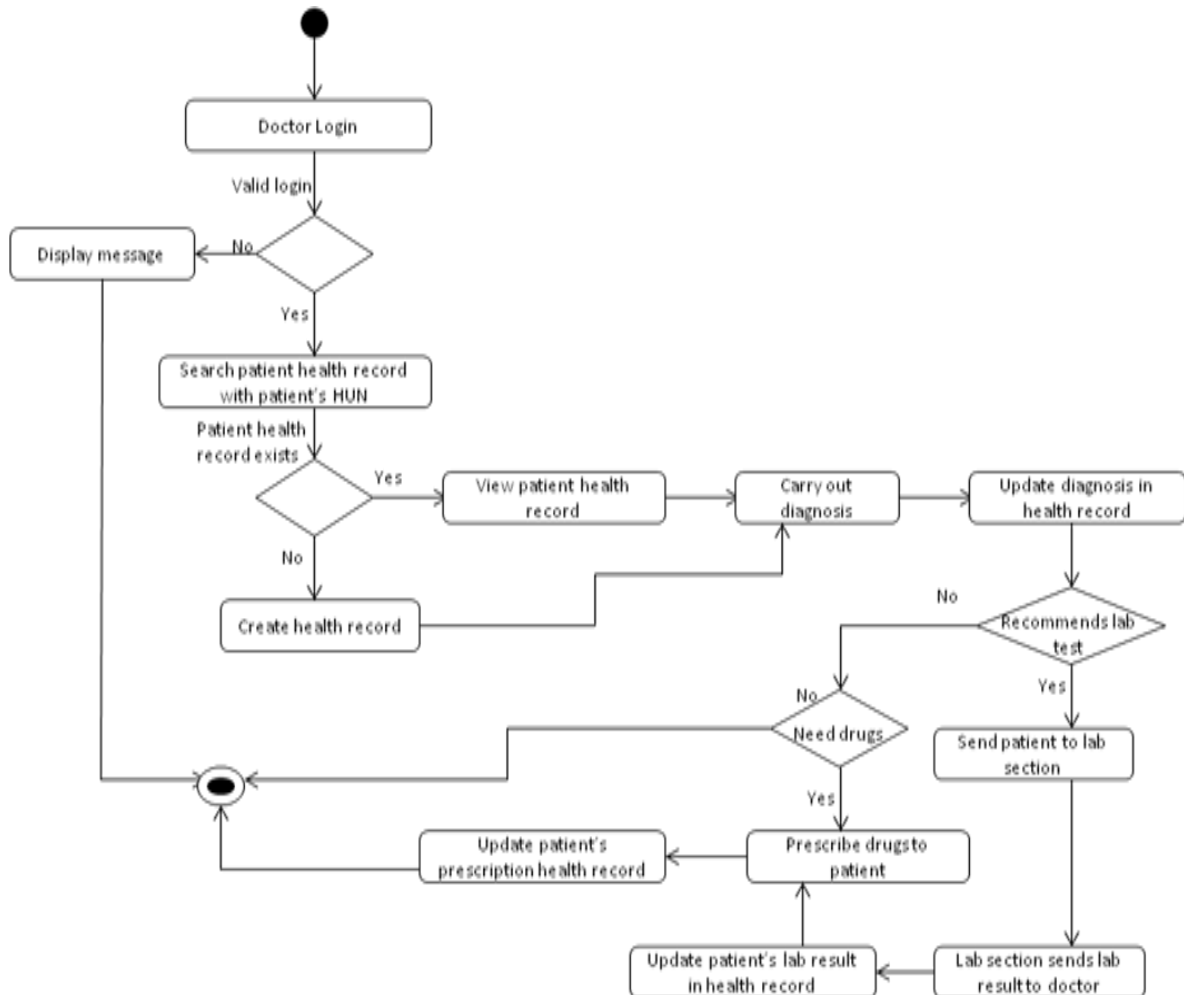
Figure 2: The Activity Diagram for the Treatment of a patient by a doctor.
