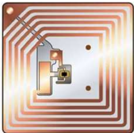
[RFID Passive Tag with antenna and microchip]
