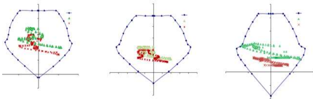
Figure 13. P-M diagrams for different sections ( E^{at} , E^{dtb} , and FZ)
