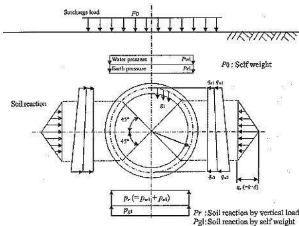
Figure 6. The distribution of loads used in JSCE [11]
