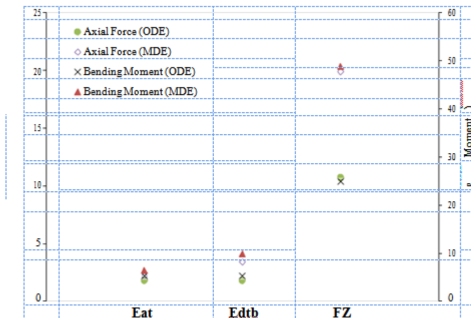
Figure 14. The axial force and bending moment in earthquake loading (ODE and MDE condition)
