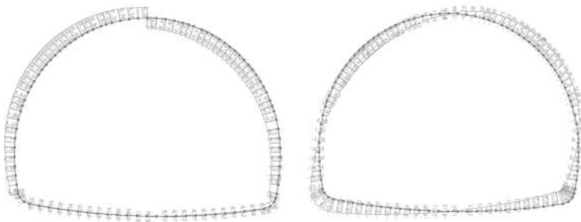
Figure 12. The state of a) axial force and b) bending moment in tunnel lining under earthquake loading (FZ section)
