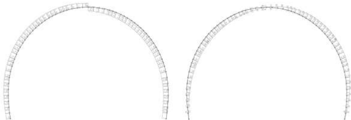
Figure 9. The state of a) axial force and b) bending moment in tunnel lining under static loading (E at section)
