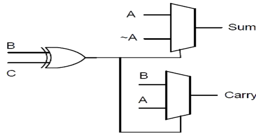
Figure 4 Proposed Full Adders
