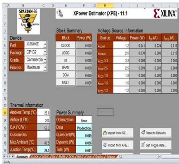
Figure 7 Power Analysis New Full Adder (NFA) Counters of System
