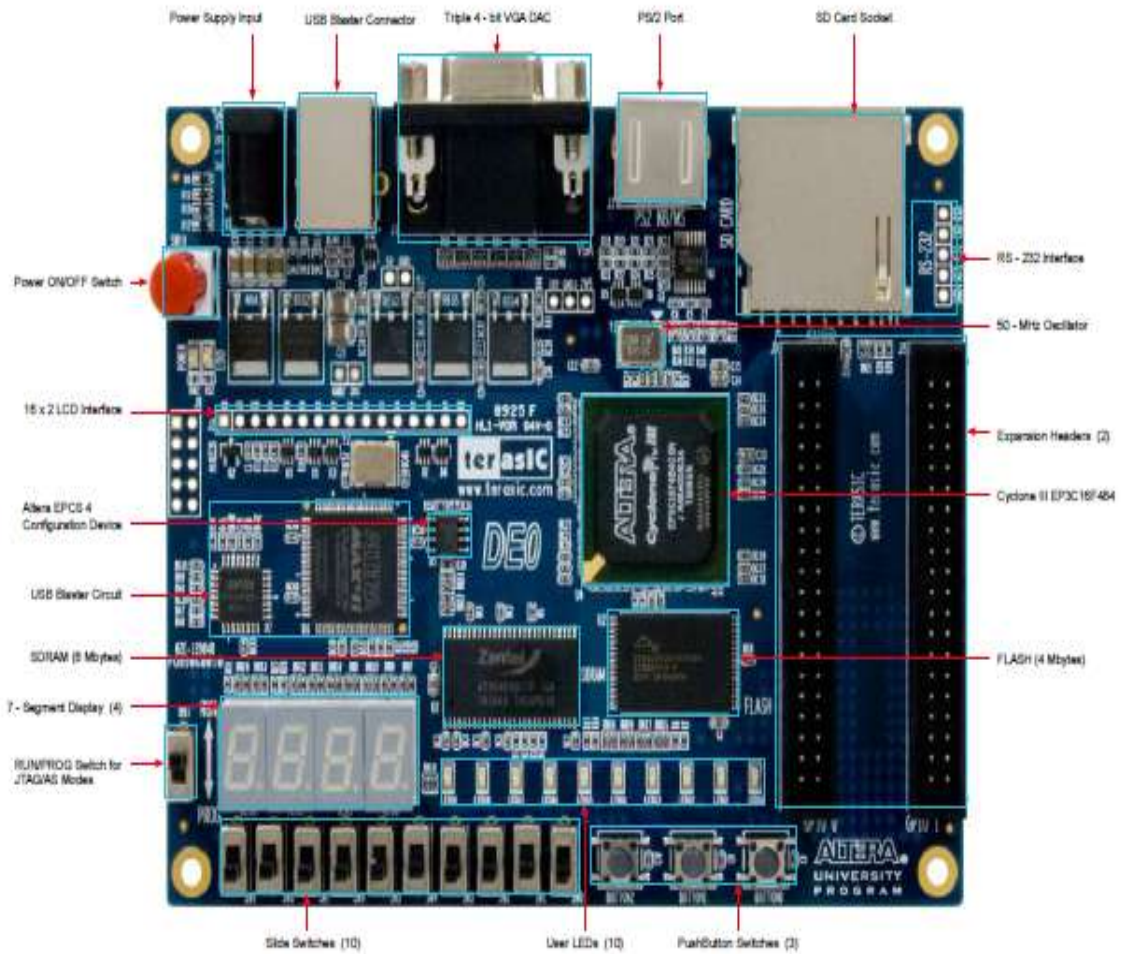
Fig . The Deo Board Samples Output
