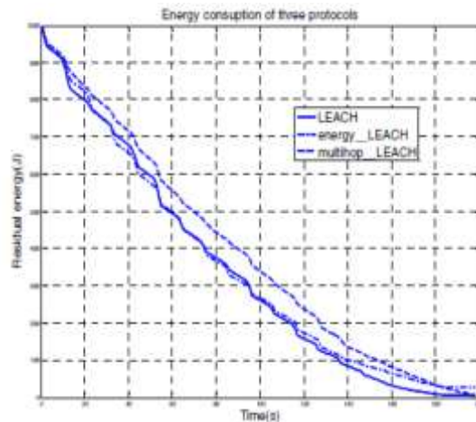
FIGURE 2: RESIDUAL ENERGY V/S TIME
