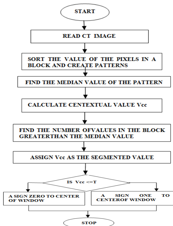
Fig. 2 Flow diagram of proposed algorithm
