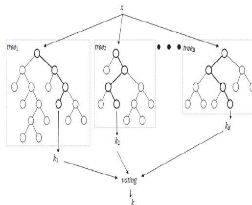
Fig. 3. Random Forest Classifier
