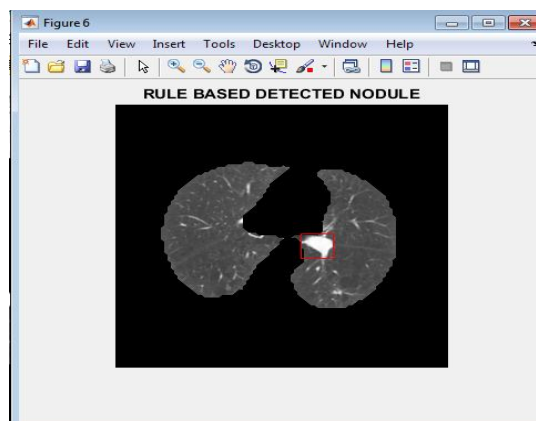
Fig. 9. Detected Nodule
