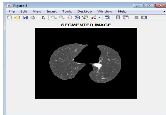
Fig. 8. Segmented Lungs
