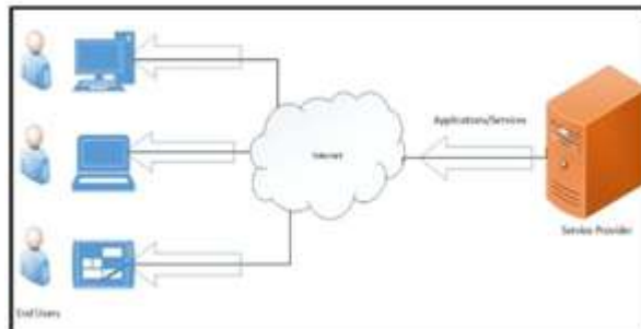
Figure 12: SaaS framework
