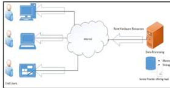
Figure 13: HaaS Framework
