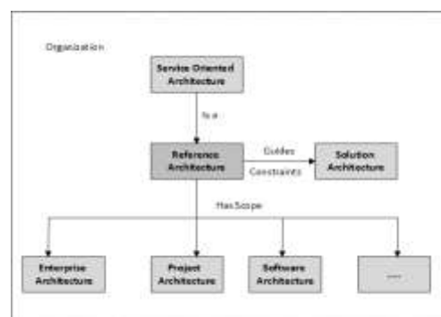
Figure 1: Architecture Model
