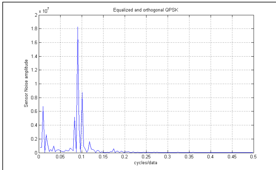
Fig2:- QPSK signal in Equalized and Orthogonal Form
