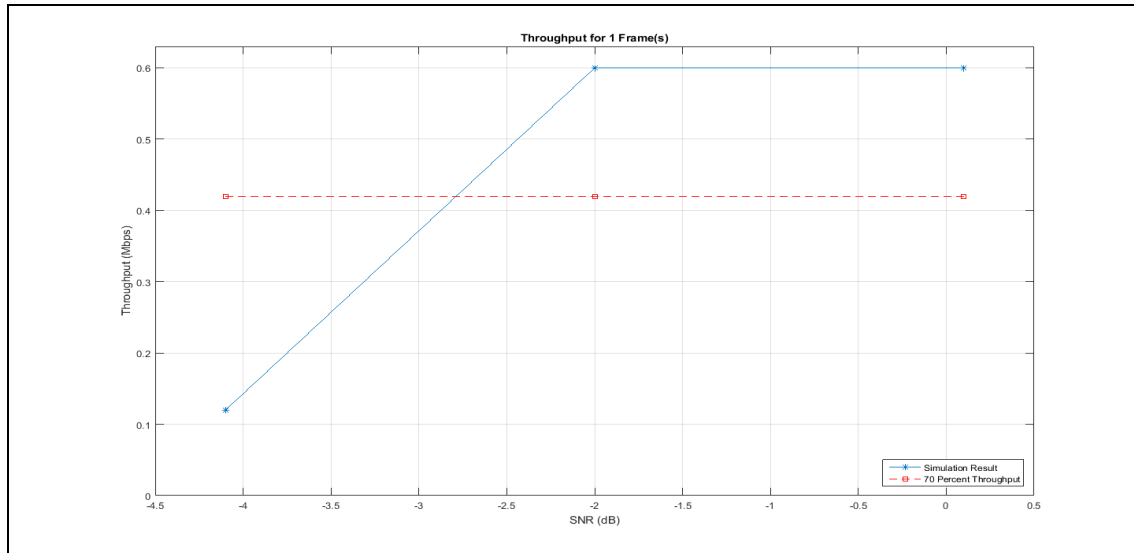
Fig6:- Throughput vs Signal to Noise Ratio
