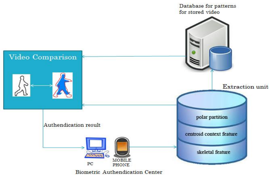
Fig1: Architecture Diagram of Video Surveillance
