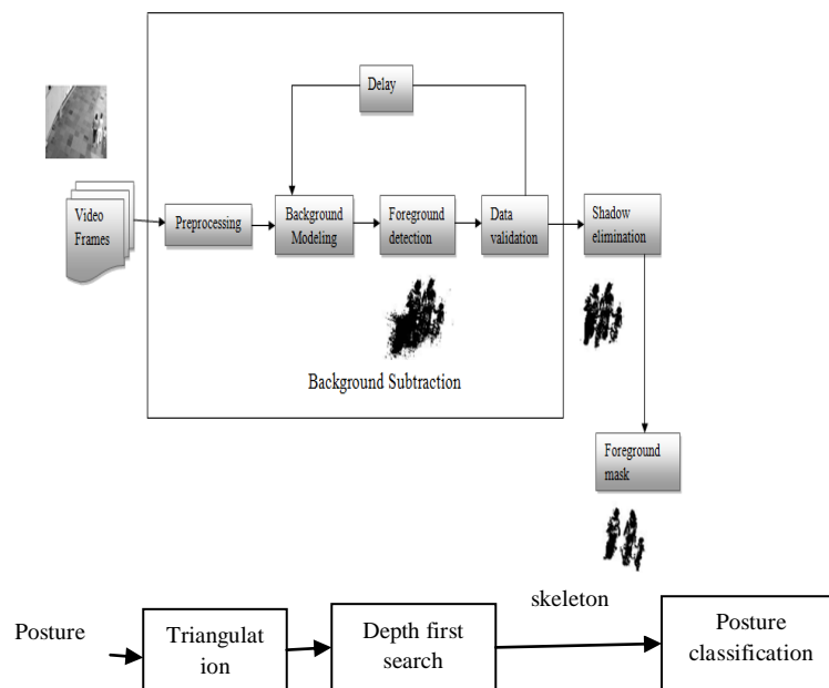
Fig 4 : Block Diagram of Steps Involved in Background Subtraction and Shadow Elimination
