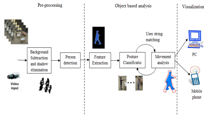
Fig 9: Block Diagram of Steps Involved in Extraction Unit and the Analysis of Movements
