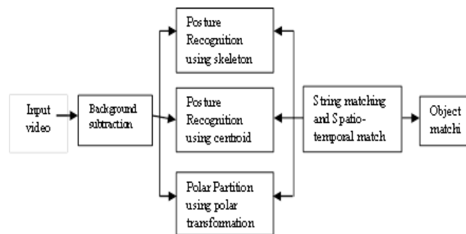
Fig 2: Flowchart of Video Surveillance
