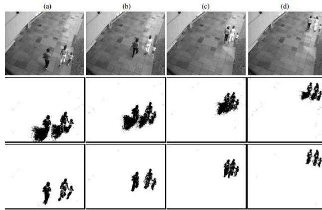
Fig 3: Top row : Frames of video sequence. Second row : Detected foreground objects. Third row : Foreground objects with shadow removal.
